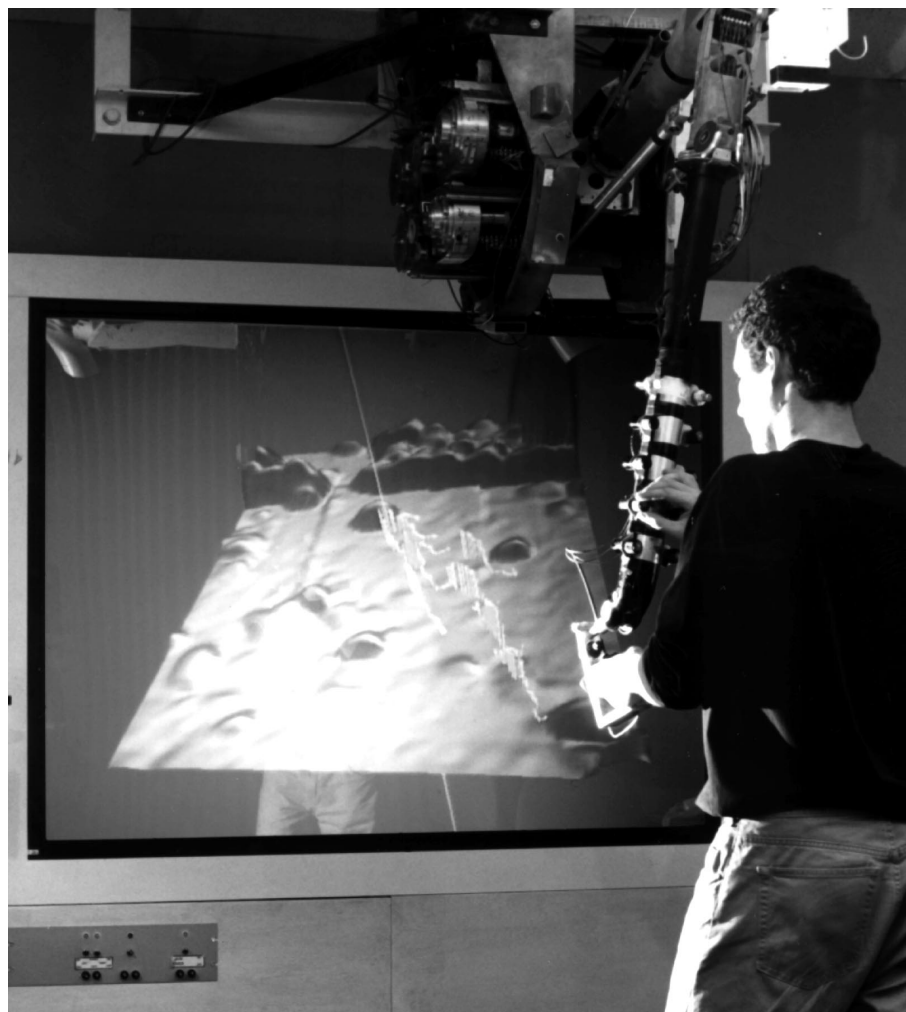
Figure 3. Using an atomic force microscope, Michael Falvo taps a gold ball into the desired gap in a circuit. (The entire field of his view is 1 nm.)
