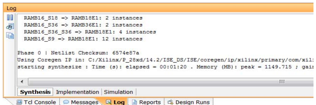
Figure 1-19: Log Window
