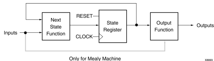
Figure 3-3: FSM Representation Incorporating Mealy and Moore Machines Diagram
