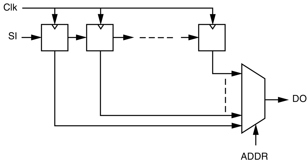
Figure 3-1: Dynamic Shift Registers Diagram
