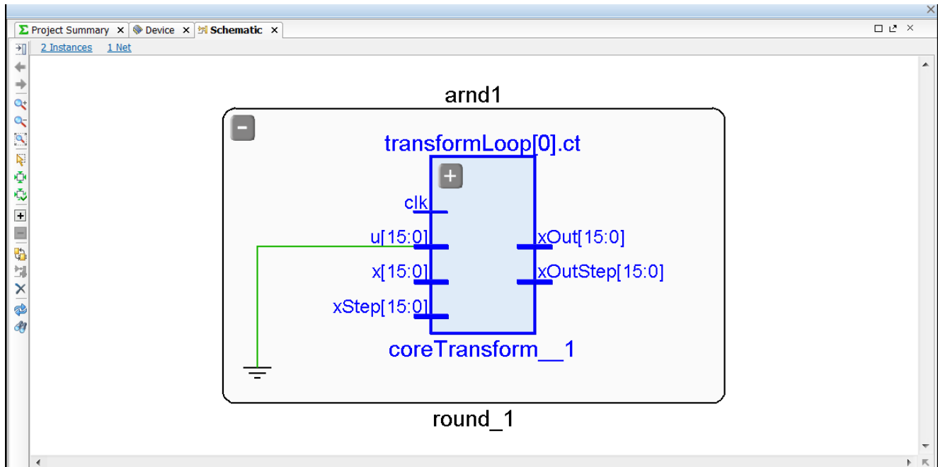
Figure 1-25: Schematic Window
