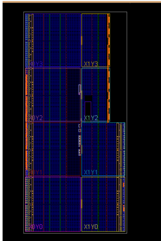
Figure 1-22: Device Window
