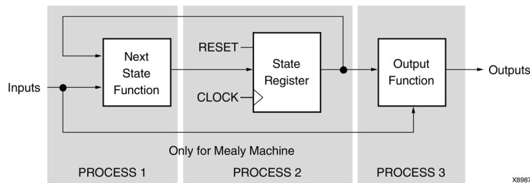
Figure 3-4: FSM With Three Processes Diagram
