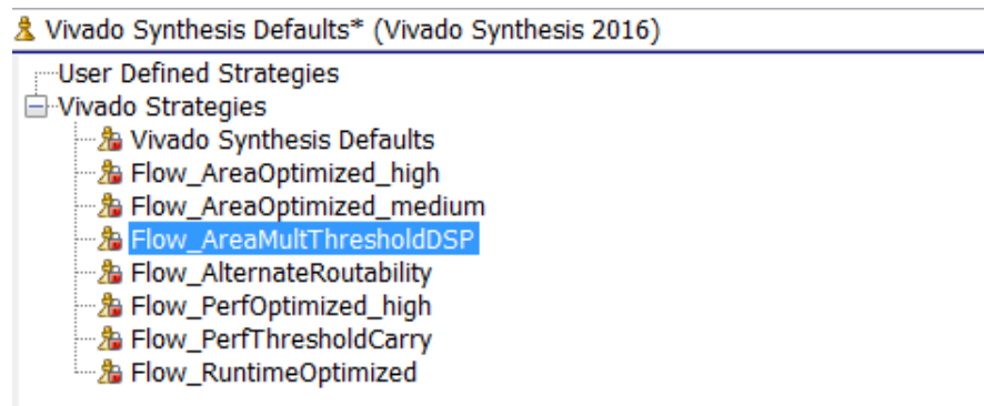
Figure 1-3: Options - Strategies
