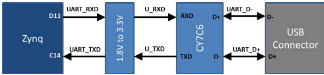
Figure 7 – USB-UART Bridge Interface
