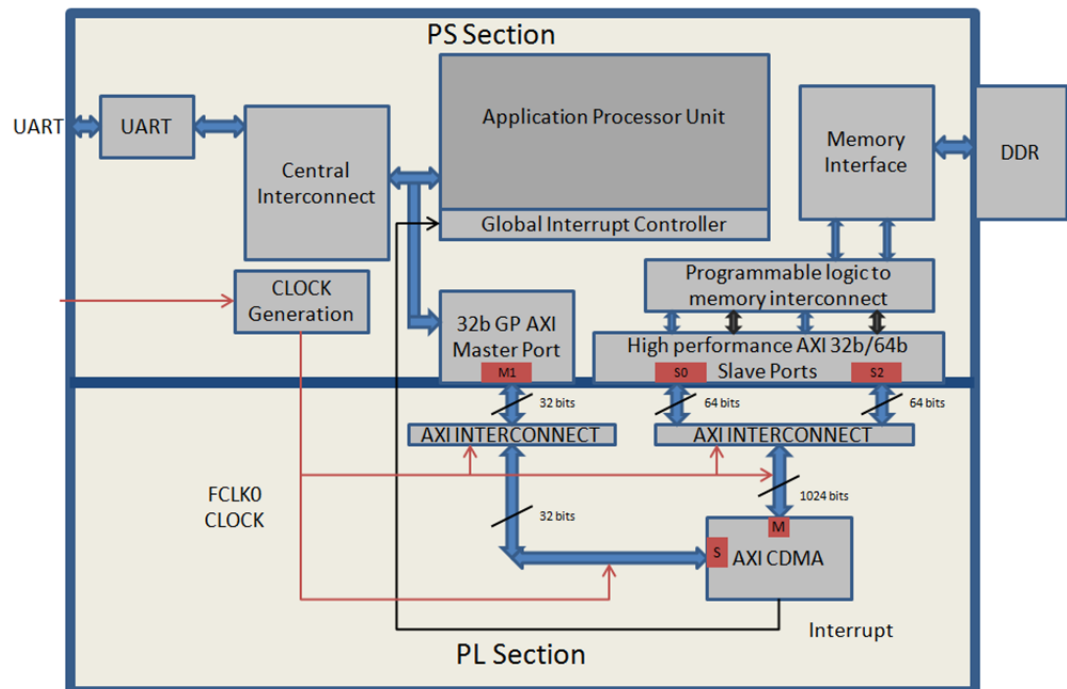
Figure 6-1: Block Diagram
