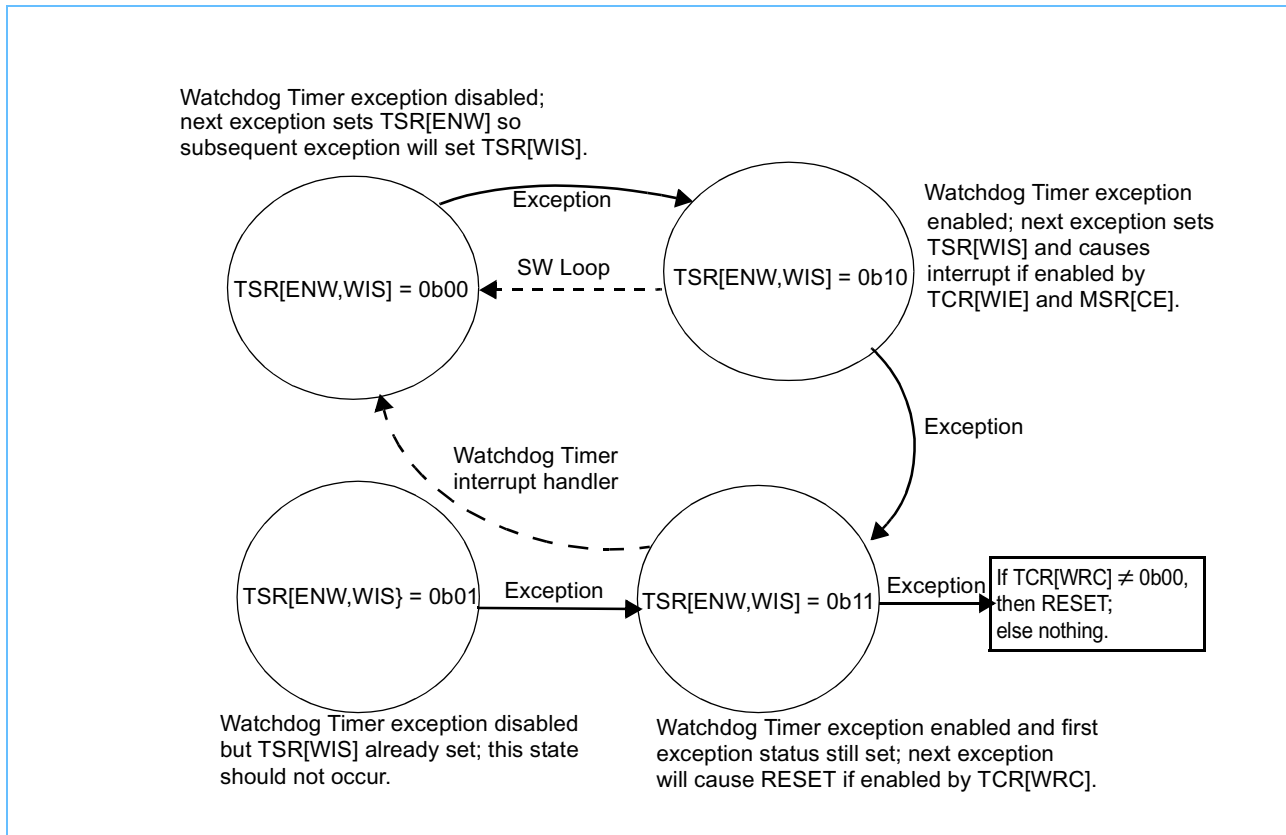
Figure 7-6. Watchdog State Machine
