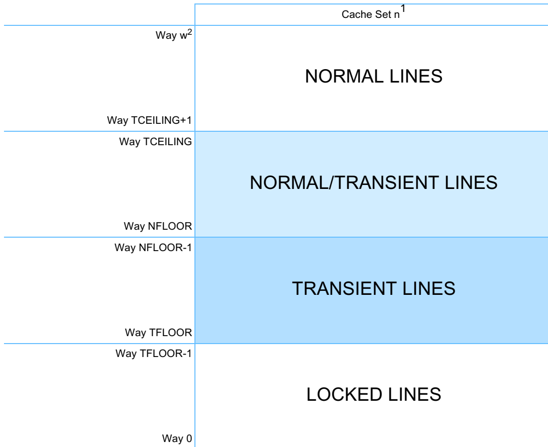
Figure 4-4. Cache Locking and Transient Mechanism (Example 2)
