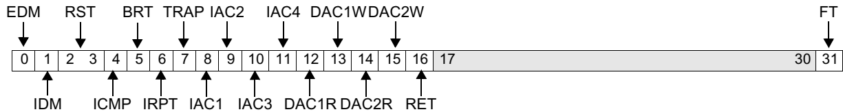
Figure 10-8. Debug Control Register 0 (DBCRO)
