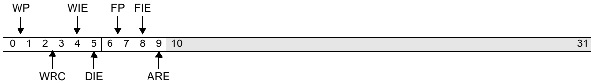
Figure 10-48. Timer Control Register (TCR)
