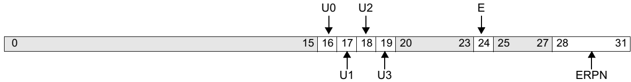
Figure 10-42. Reset Configuration
