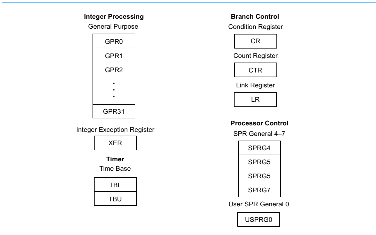
Figure 2-1. User Programming Model Registers
