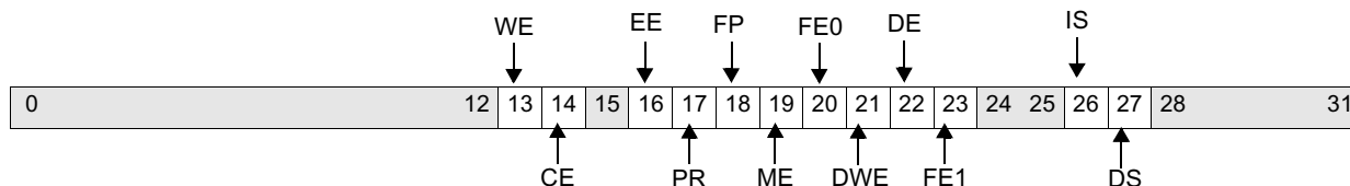
Figure 6-3. Save/Restore Register 1 (SRR1)
