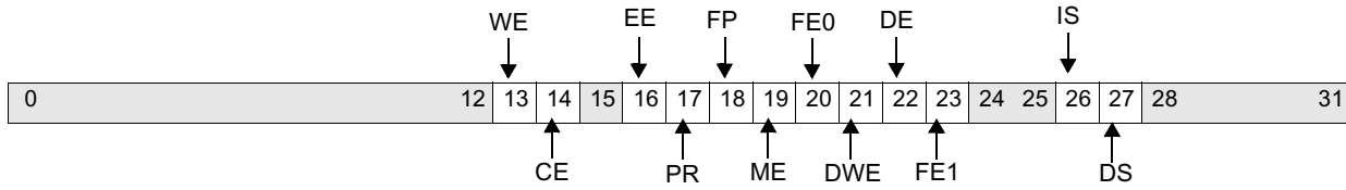
Figure 10-36. Machine Check Save/Restore Register 1 (MCSRR1)
