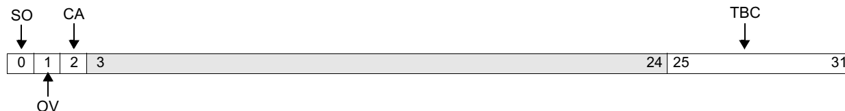
Figure 10-51. Integer Exception Register (XER)
