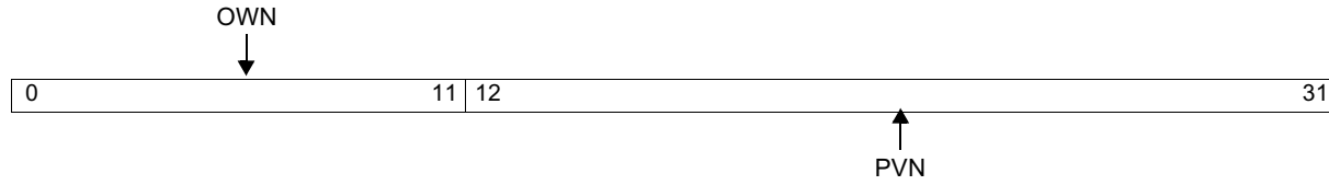
Figure 10-41. Processor Version Register (PVR)
