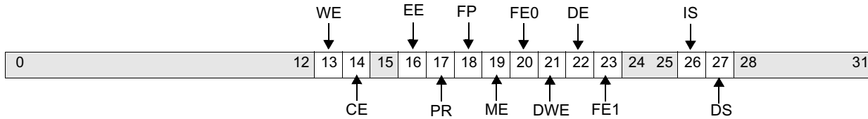
Figure 10-38. Machine State Register (MSR)
