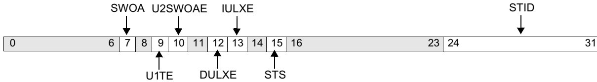
Figure 10-37. Memory Management Unit Control Register (MMUCR)
