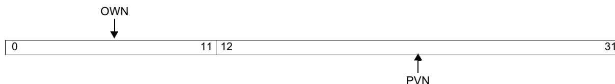
Figure 2-9. Processor Version Register (PVR)
