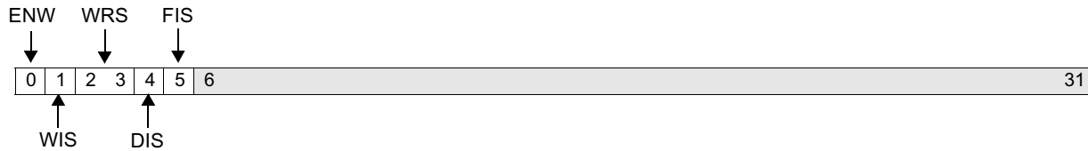
Figure 10-49. Timer Status Register (TSR)
