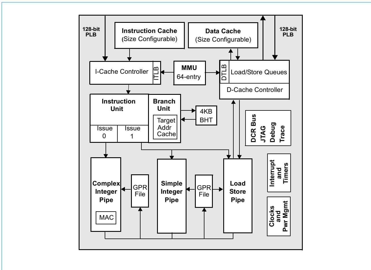
Figure 1-1. PPC440x5 Core Block Diagram
