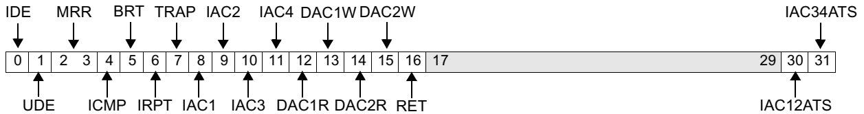
Figure 8-4. Debug Status Register (DBSR)
