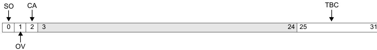
Figure 2-7. Integer Exception Register (XER)
