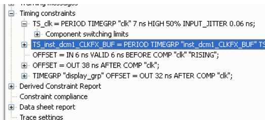
Figure 5-18: Selecting Post-Map Static Timing Constraint
