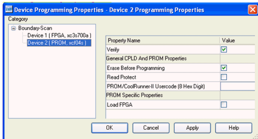
Figure 7-8: Program Options for XC3S700A Device
