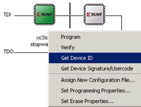
Figure 7-13: Selecting a Boundary-Scan Operation
