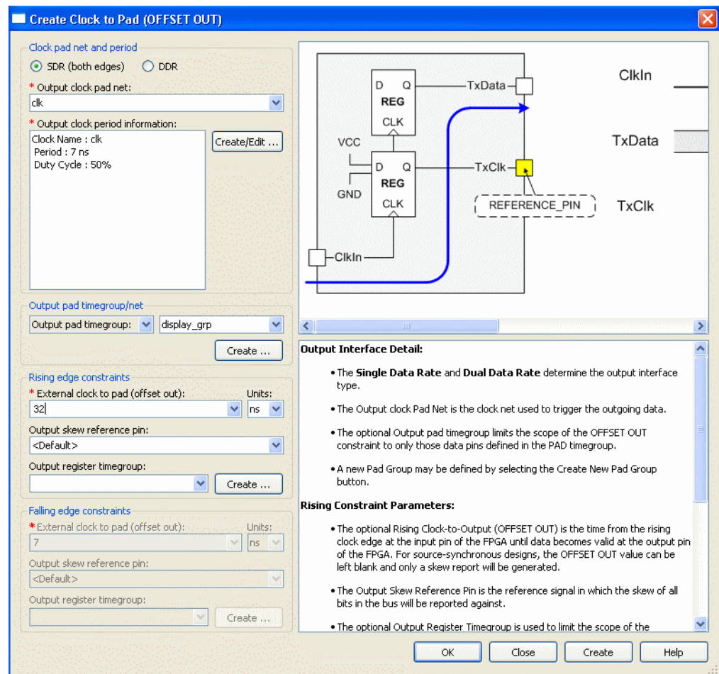
Figure 5-10: Clock to Pad Dialog Box
