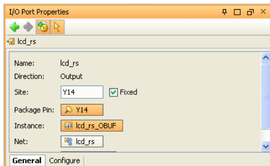
Figure 5-14: Assigning I/O Pins Using I/O Port Properties
