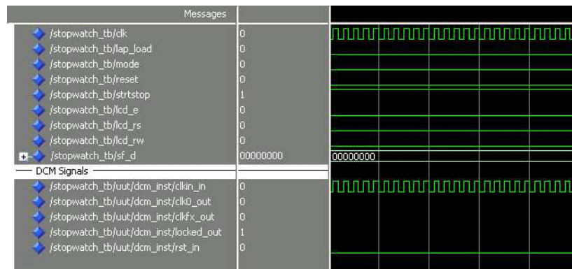
Figure 4-6: Waveform After Adding DCM Signals Divider
