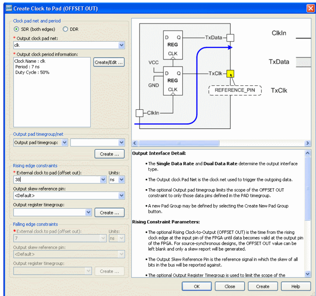
Figure 5-8: Offset Out Constraint
