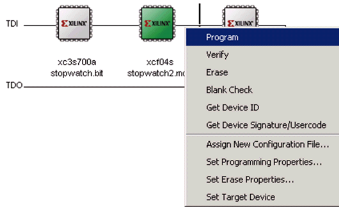
Figure 7-15: Available Boundary-Scan Operations for XCF02S Device
