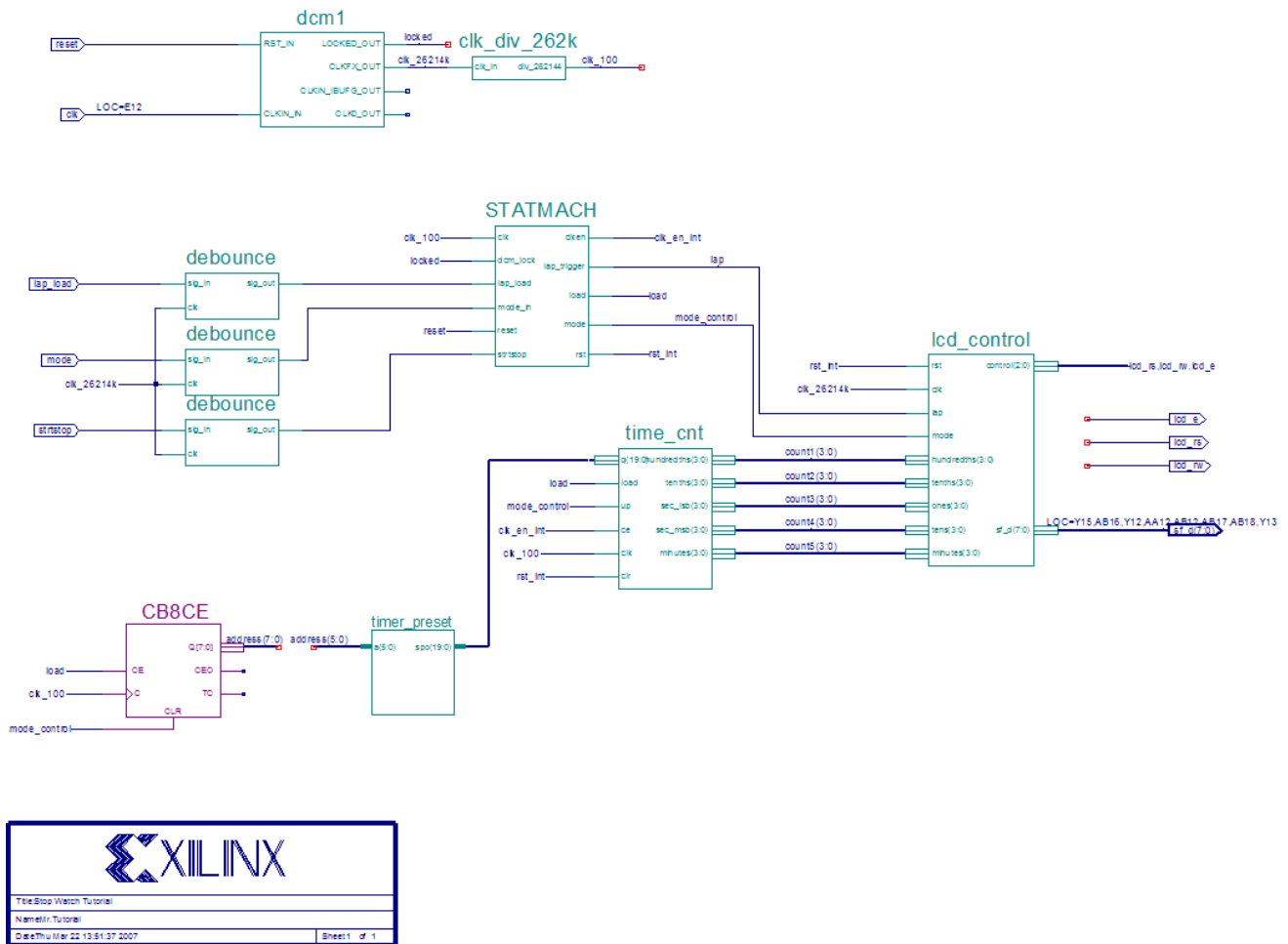
Figure 3-31: Completed Stopwatch Schematic
