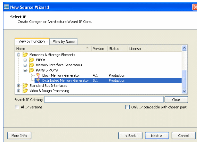
Figure 2-11: New Source Wizard—Select IP Page
