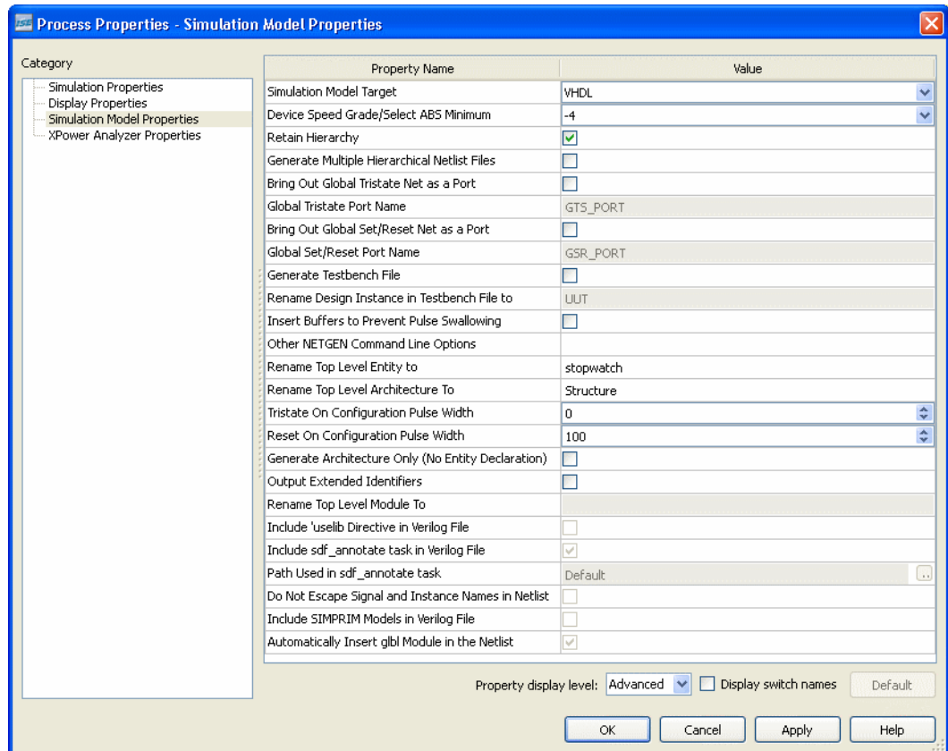
Figure 6-1: Simulation Model Properties
