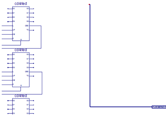
Figure 3-10: Adding a Bus
