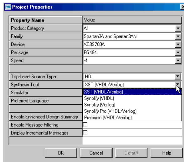
Figure 2-24: Specifying Synthesis Tool
