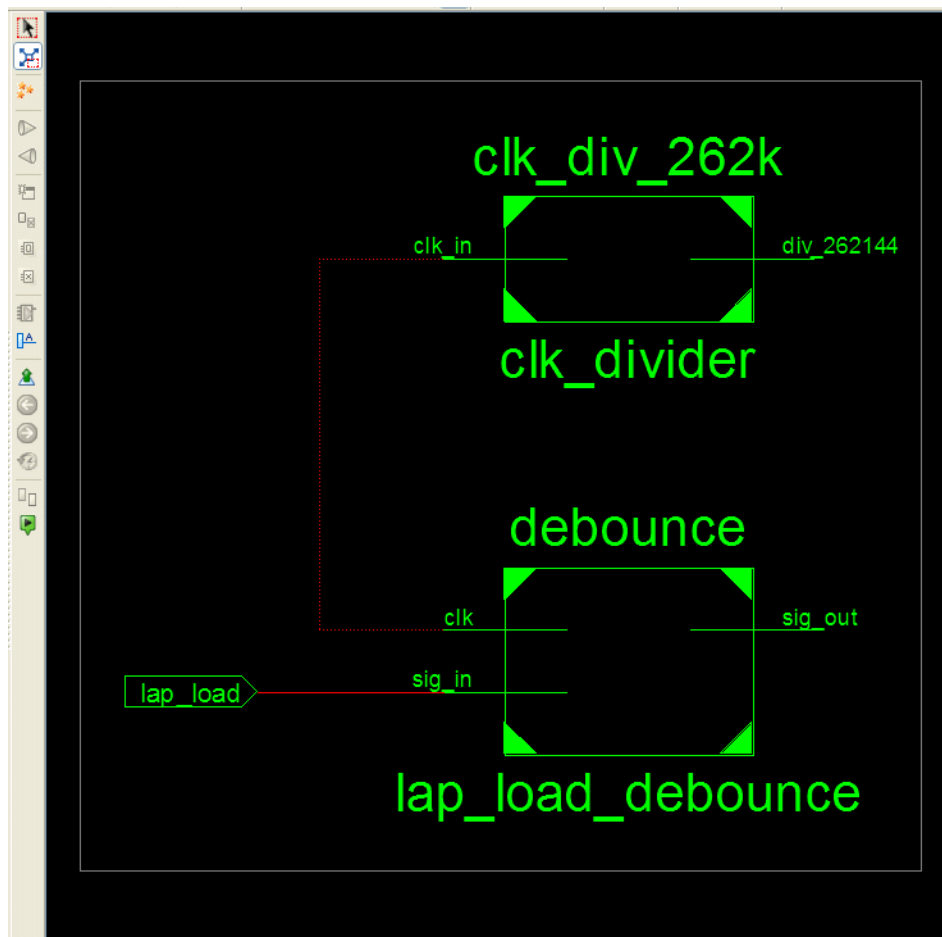
Figure 2-26: RTL Schematic
