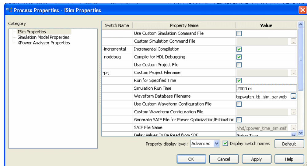
Figure 6-11: Simulation Properties
