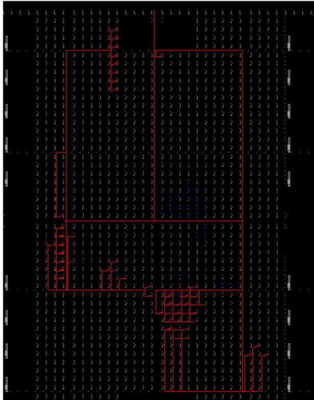
Figure 5-22: Clock Net
