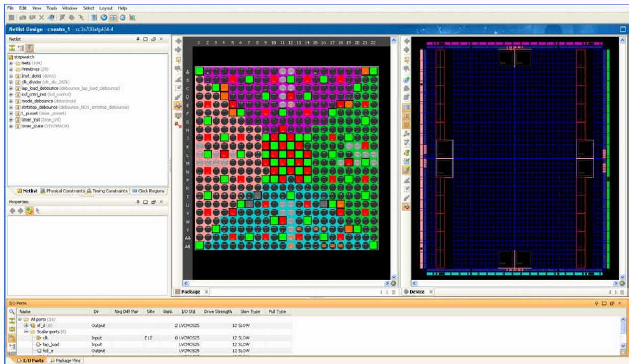
Figure 5-12: PlanAhead Software for I/O Planning
