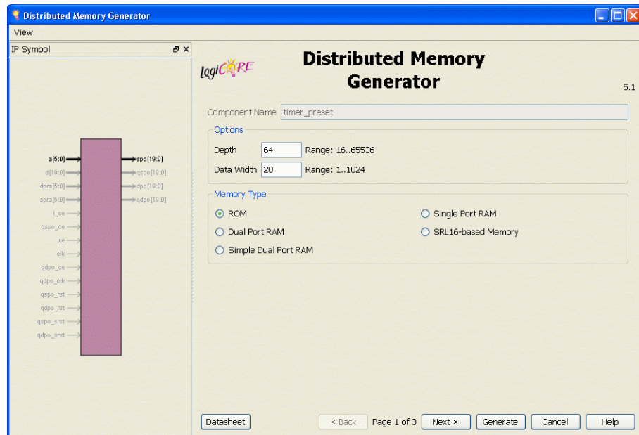
Figure 2-12: CORE Generator Software—Distributed Memory Generator Customization GUI Page 1
