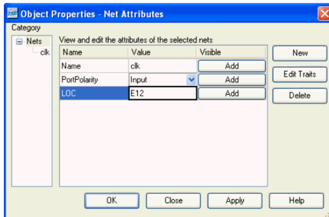
Figure 3-30: Assigning Pin Locations
