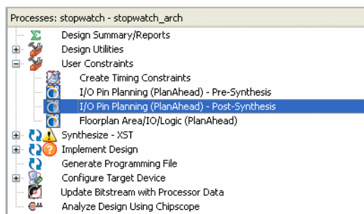
Figure 5-11: I/O Pin Planning—Post-Synthesis
