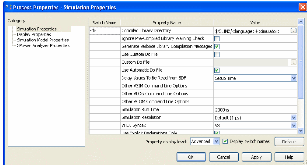
Figure 6-2: Simulation Properties
