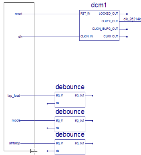
Figure 3-29: Adding I/O Markers to Labeled Nets
