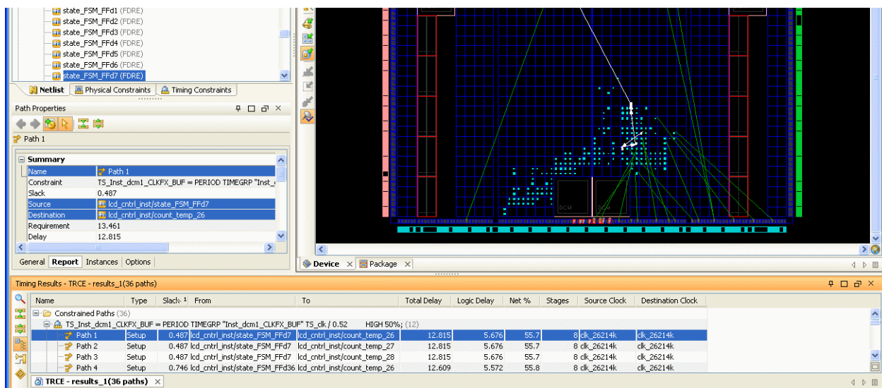
Figure 5-24: Viewing Timing Path in PlanAhead Software
