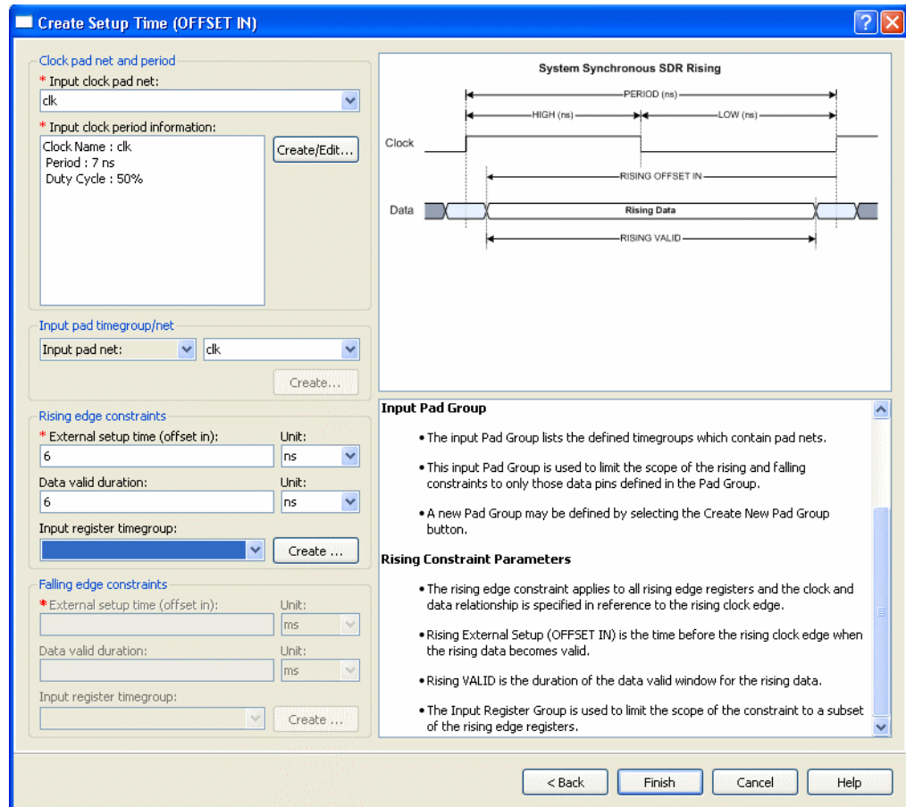
Figure 5-7: Offset In Constraint—Page 2
