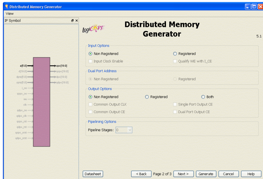
Figure 2-13: CORE Generator Software—Distributed Memory Generator Customization GUI Page 2
