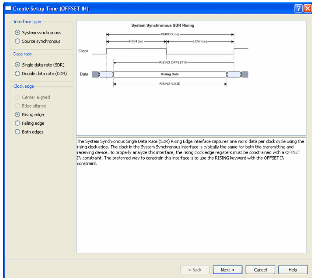
Figure 5-6: Offset In Constraint—Page 1
