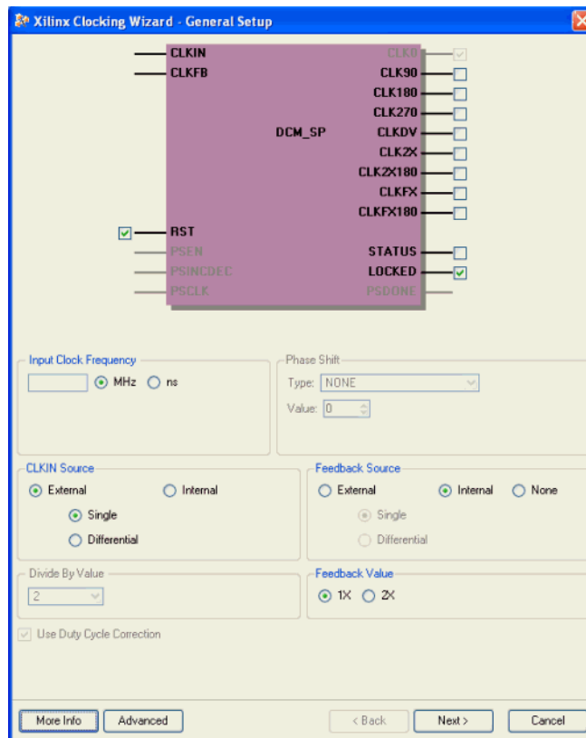
Figure 3-19: Xilinx Clocking Wizard—General Setup
