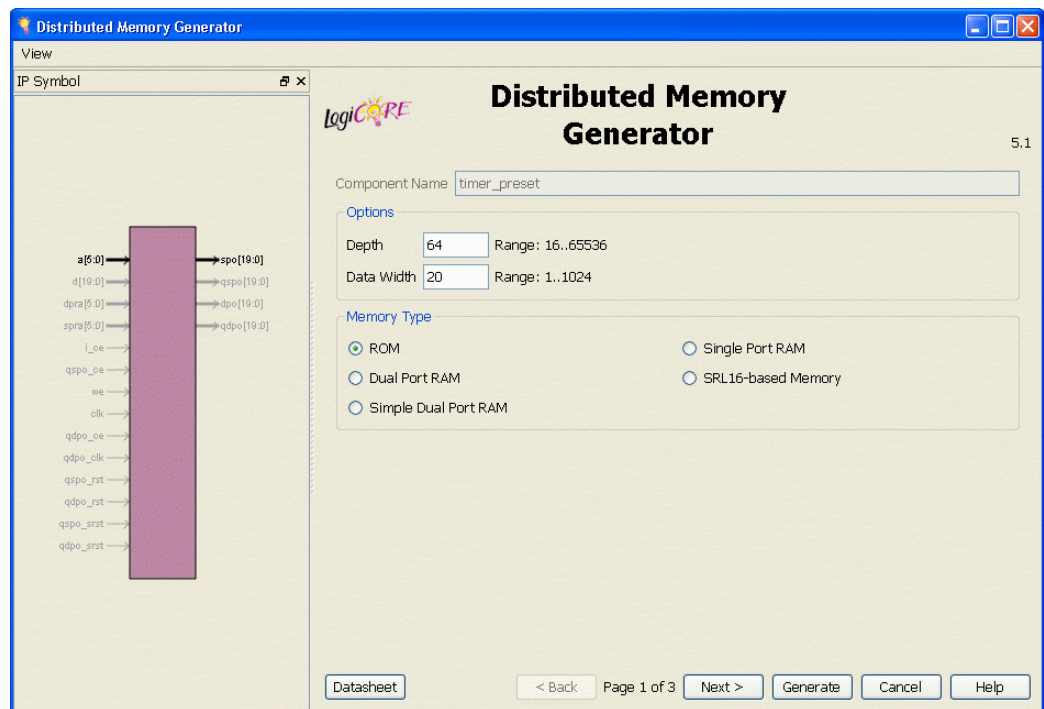
Figure 3-17: CORE Generator Software—Distributed Memory Generator Customization GUI
