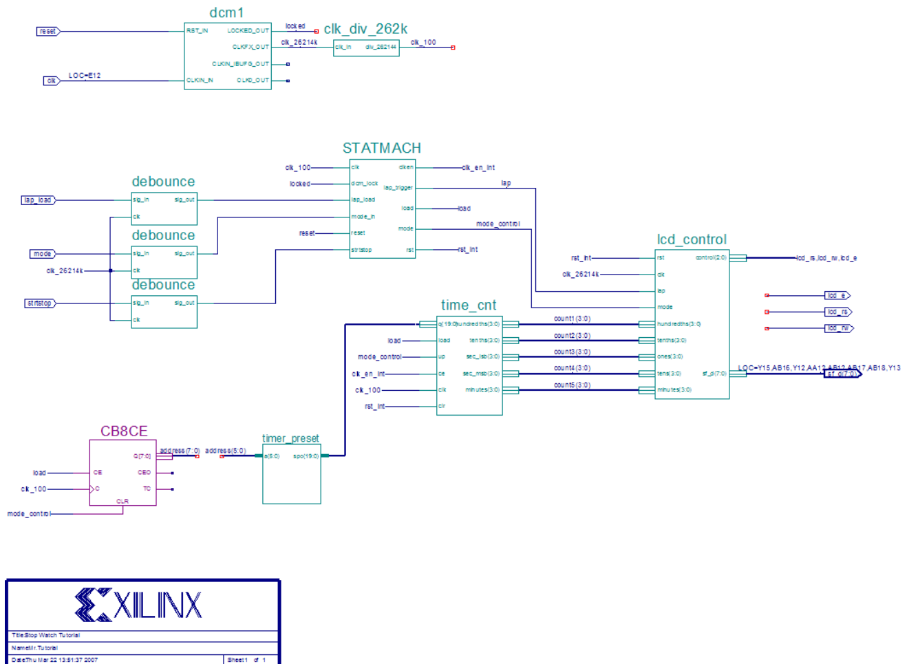
Figure 3-2: Completed Stopwatch Schematic
