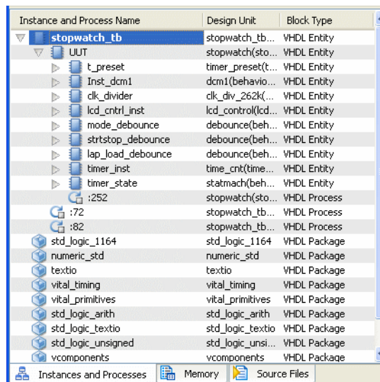
Figure 4-12: Simulation Hierarchy—VHDL flow
