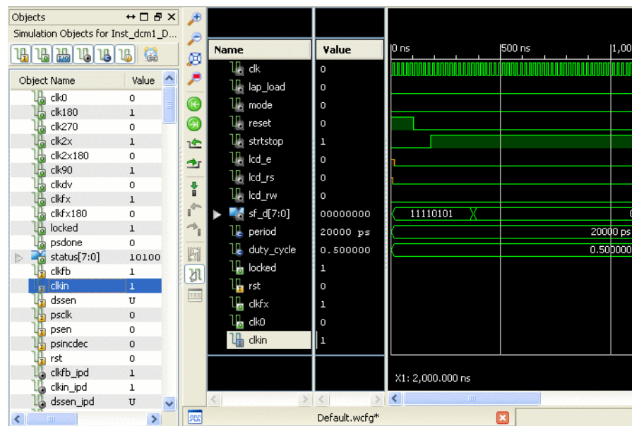
Figure 6-13: Resulting Waveform
