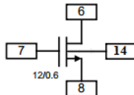
Short Channel Transistors
