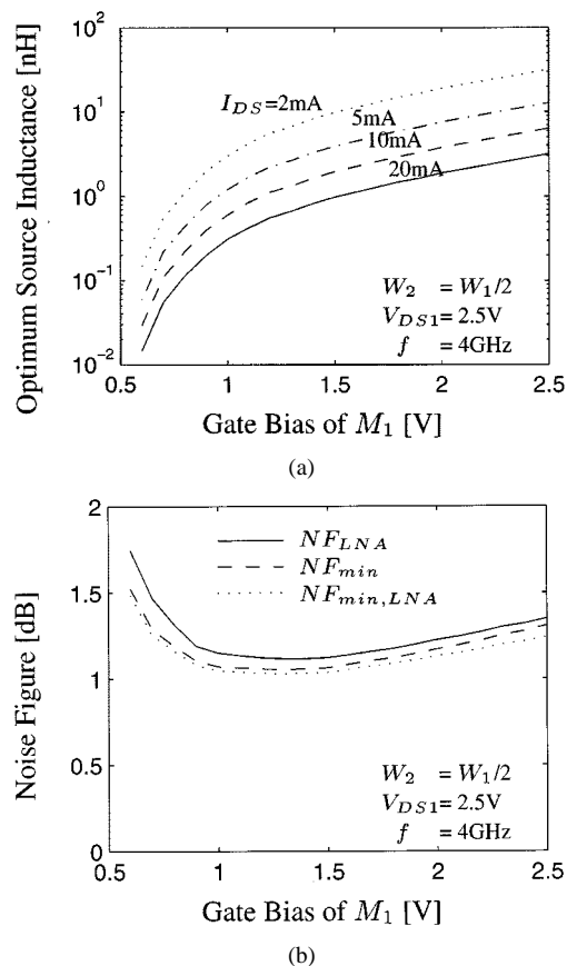
Fig. 4. (a) Optimum L_s yielding the best noise figure of the LNA for the given bias condition under the power constraint. (b) Best noise figure of the LNA with optimum L_s . The noise contributions of M_1 substrate and M_2 are excluded and C_p = 0 .
