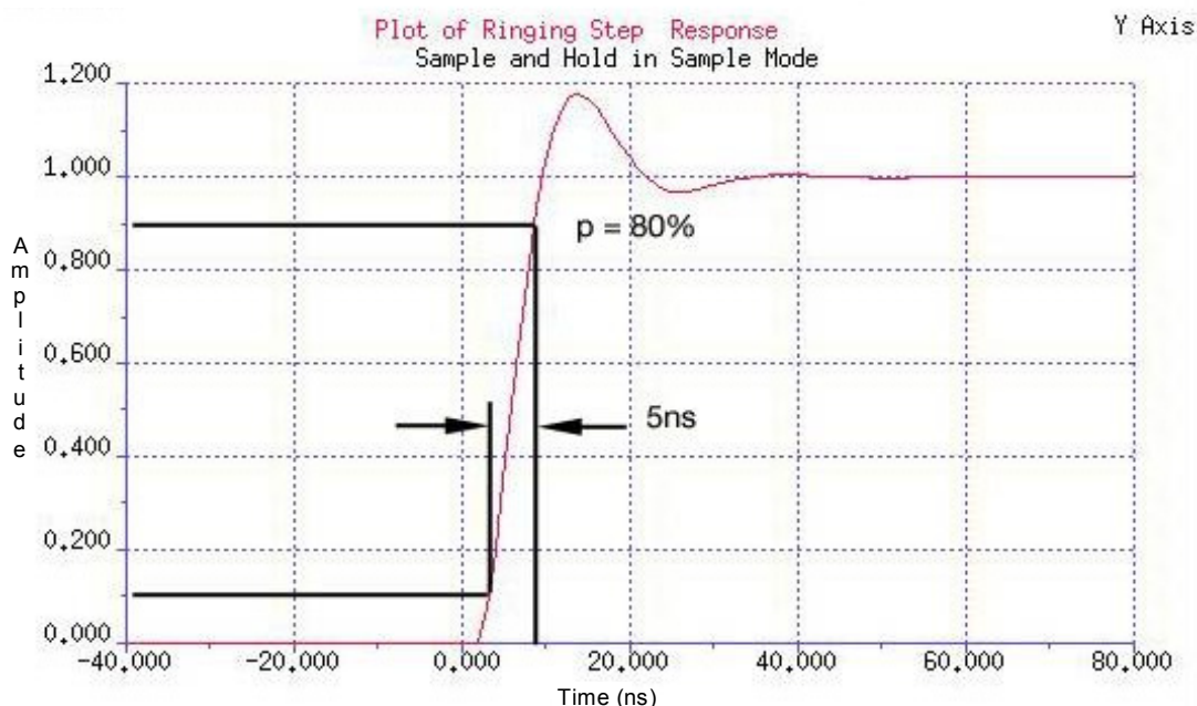
Figure 28—Ringing step response
