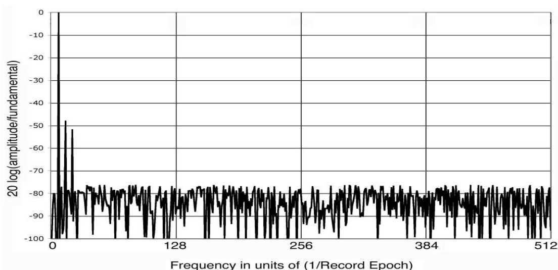
Figure D.5—Plot of the magnitude of the spectrum of the signal shown in Figure D.4
