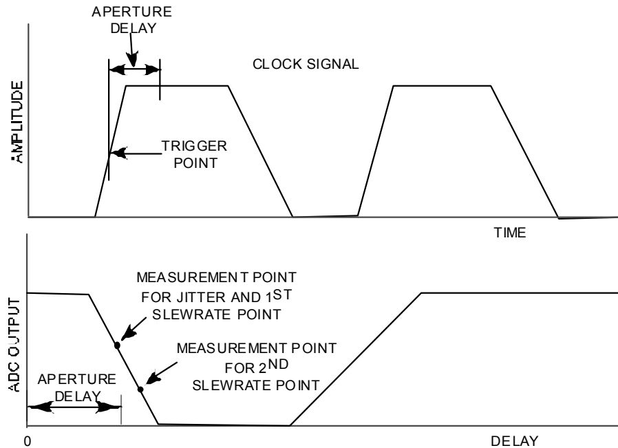
Figure 31 —The upper graph shows the clock signal as a function of time; the lower graph shows the ADC output as a function of the variable delay
