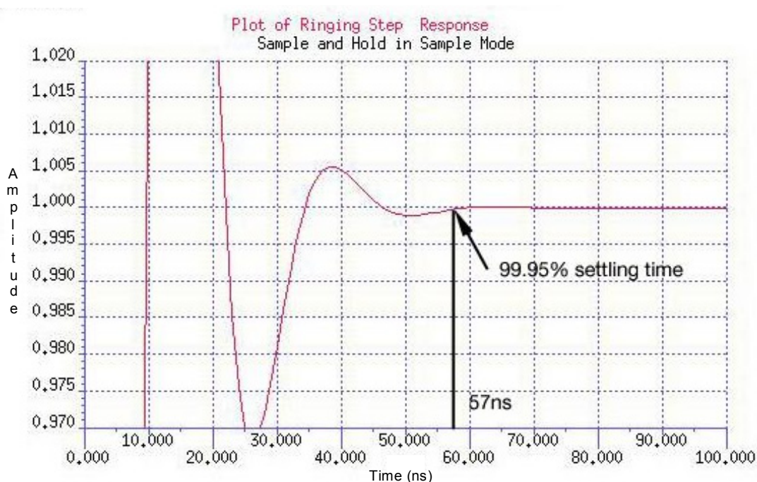
Figure 29—Zoomed ringing transition
