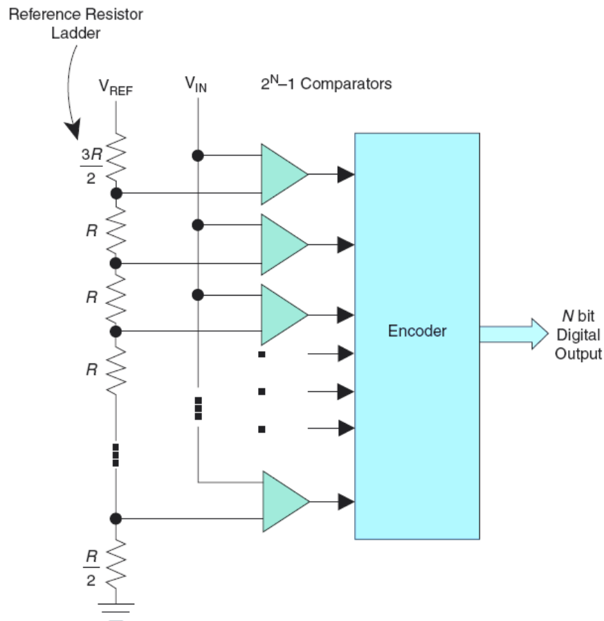
Figure A.2—Block scheme of a flash ADC
