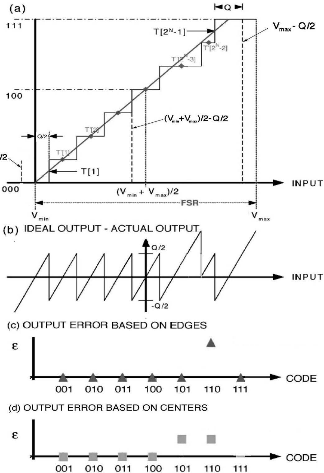
Figure 2—Methods for characterizing the error of an ADC
