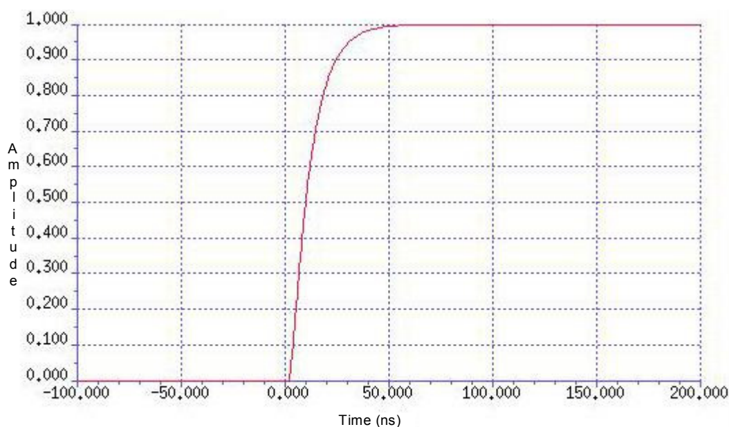
Figure 23—The step response corresponding to the impulse response of the previous figure
