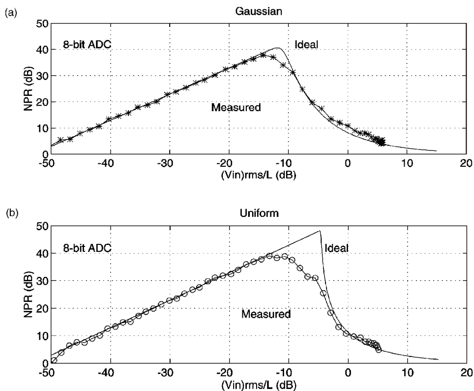
Figure 19—(a) Plot of ideal and measured NPR for a Gaussian noise input from Equation (63); (b) Plot of ideal and measured NPR for a uniform noise input from Equation (64)
