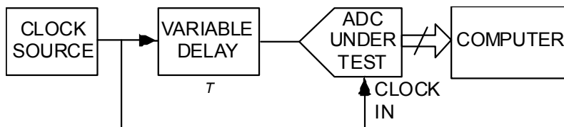
Figure 30—Test setup for aperture jitter test method; T is the value of the delay
