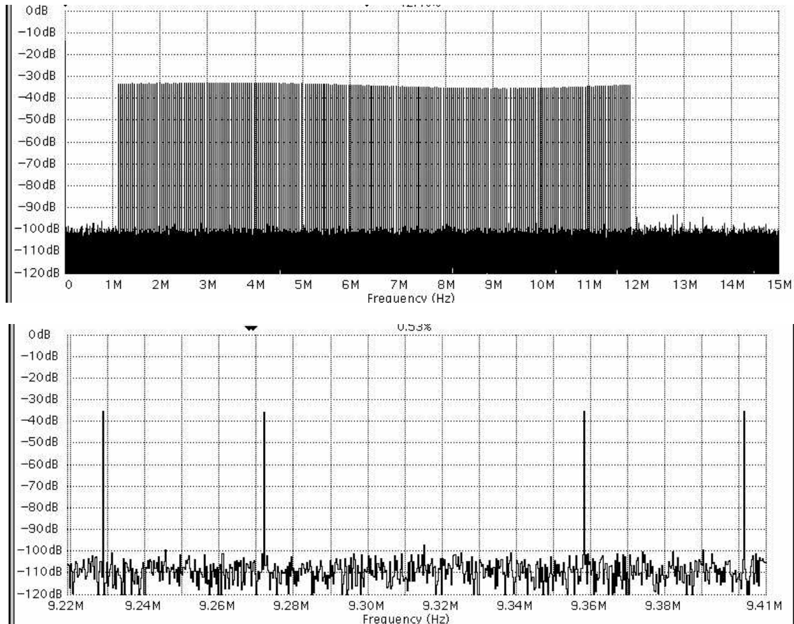
Figure 16—Full power spectrum of a multi-tone for MTPR test (upper) and close-up around a missing tone (lower)
