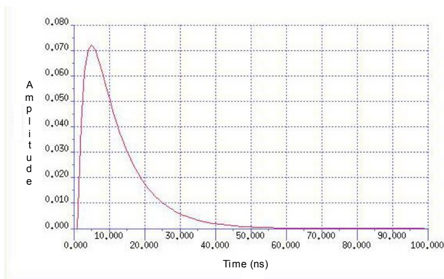
Figure 22—Impulse response of a sample-and-hold amplifier while in the sample mode
