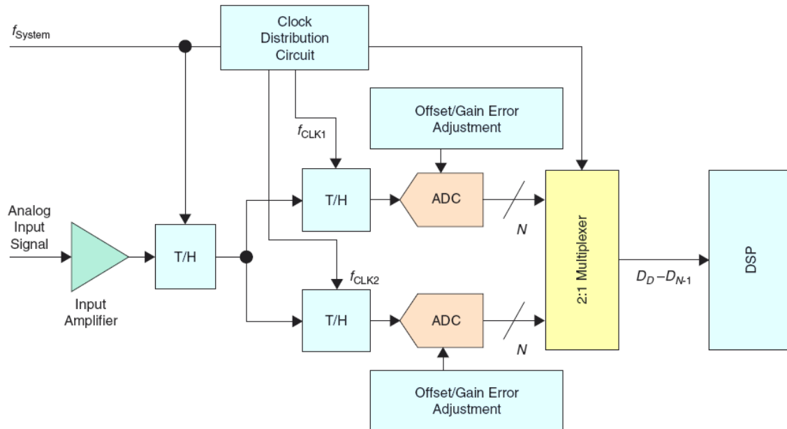
Figure A.7—Time-interleaved data acquisition system
