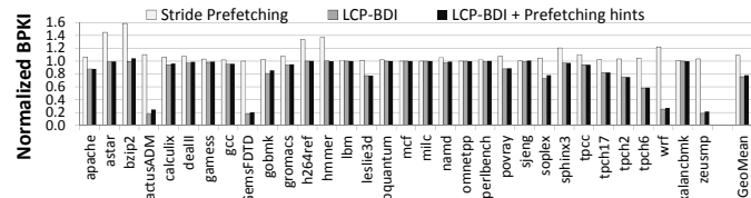
Figure 18: Bandwidth comparison with stride prefetching.
