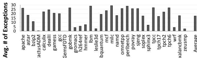
Figure 16: Average number of exceptions per compressed page for different applications.
