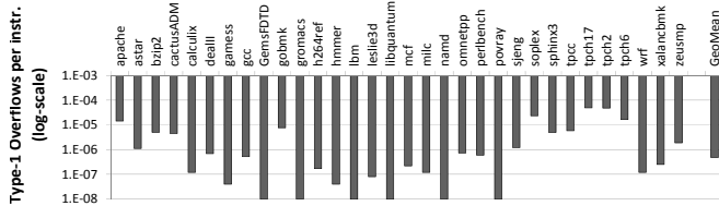
Figure 15: Type-1 page overflows for different applications.
