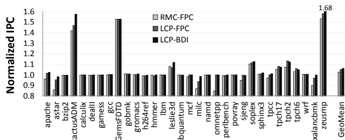
Figure 11: Performance comparison (IPC) of different compressed designs for the single-core system.
