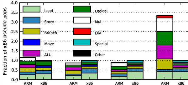
Figure 6. Selected Instruction Counts (Emulated).
